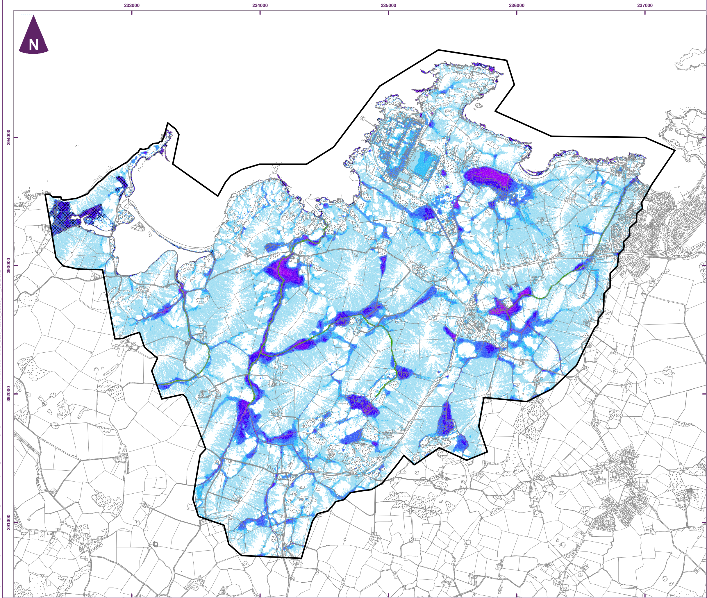
Figure 22 DCO baseline peak pluvial depth 1:1000 year AEP 60 min duration climate change 2080s - reasonably foreseeable
