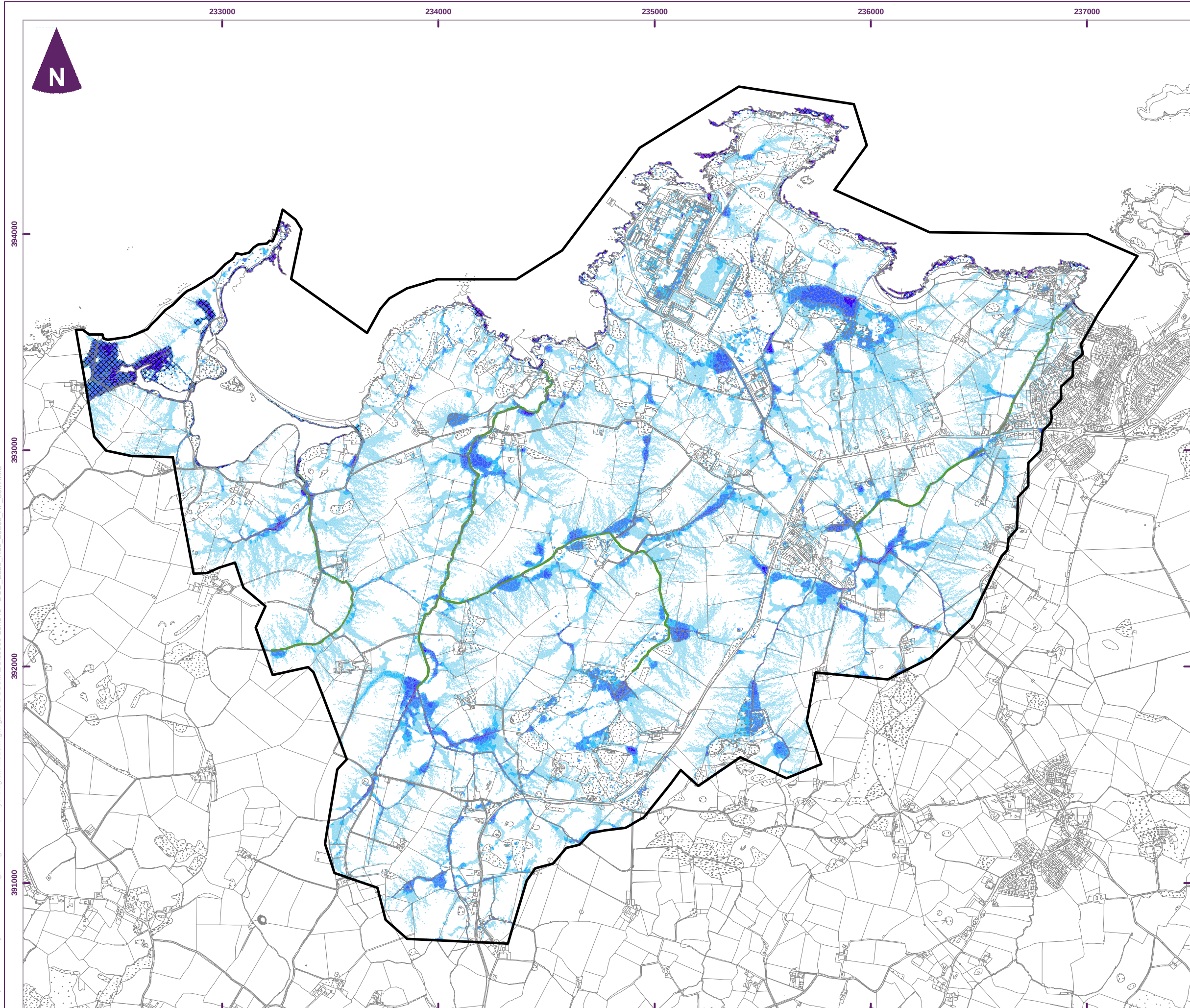
Figure 16 DCO baseline peak pluvial depth 1:30 year AEP 30 min duration climate change 2080s - reasonably foreseeable
