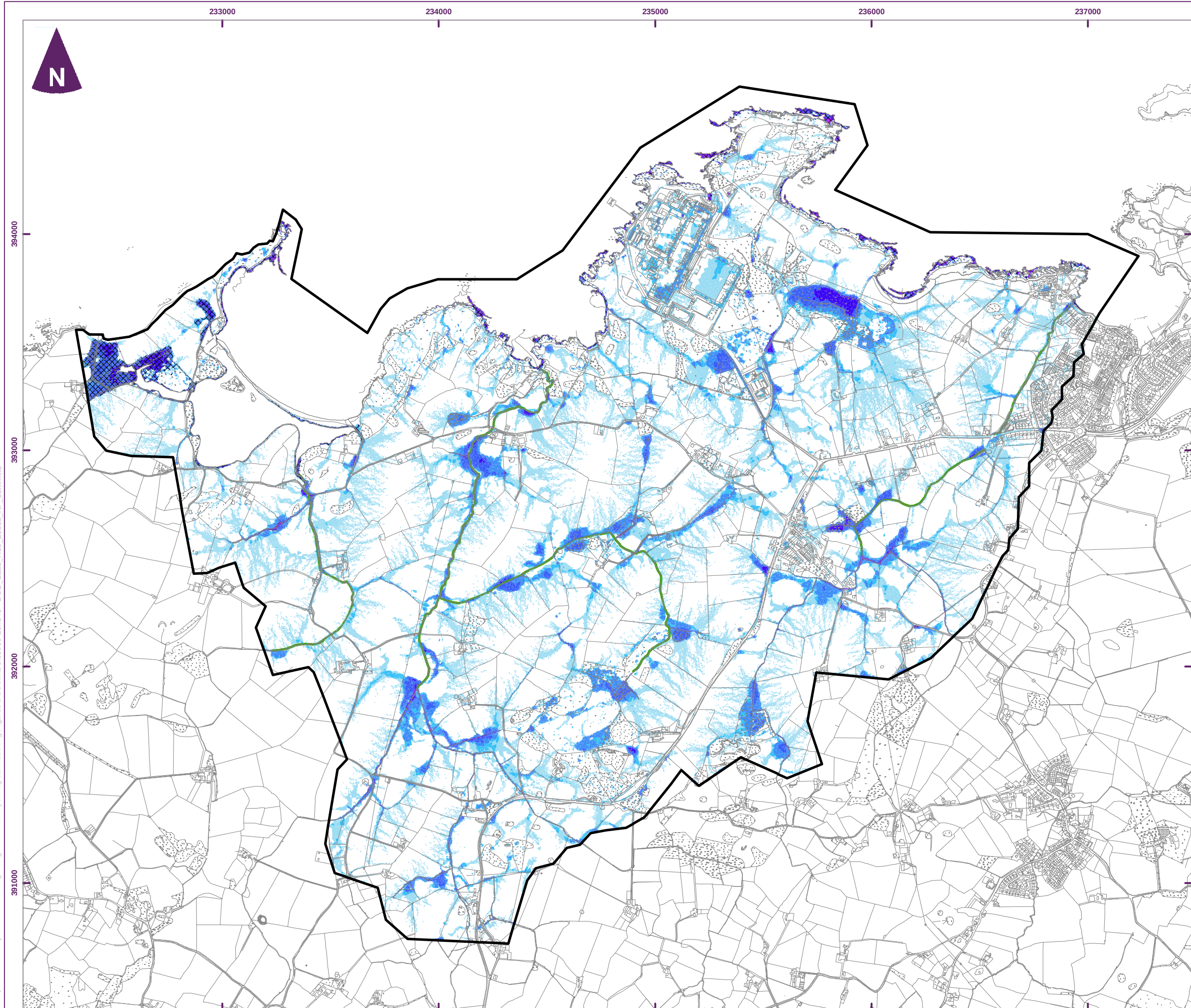
Figure 20 DCO baseline peak pluvial depth 1:30 year AEP 60 min duration climate change 2080s - reasonably foreseeable
